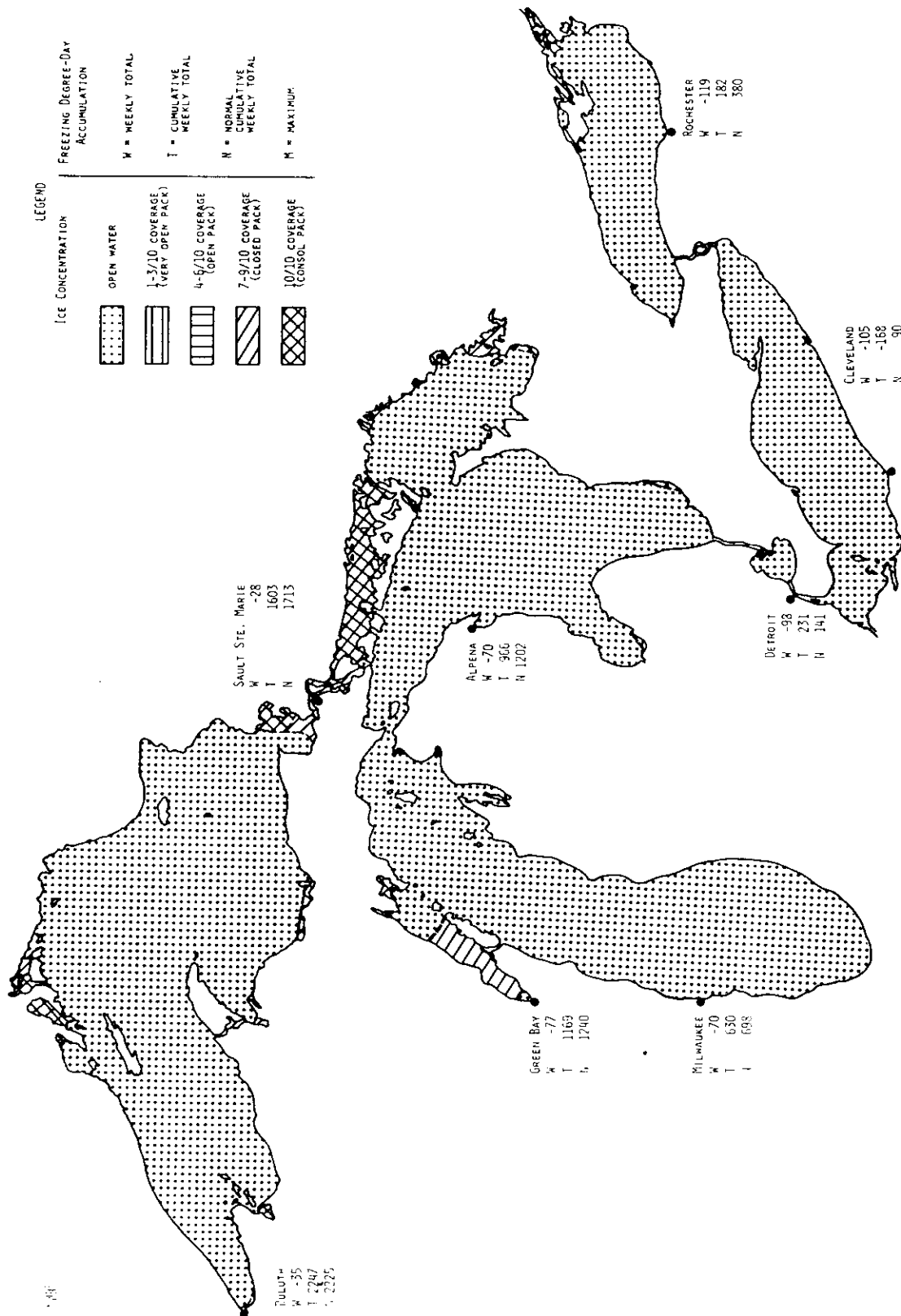
Figure A.24. Composite ice chart - week ending April 20, 1975.
