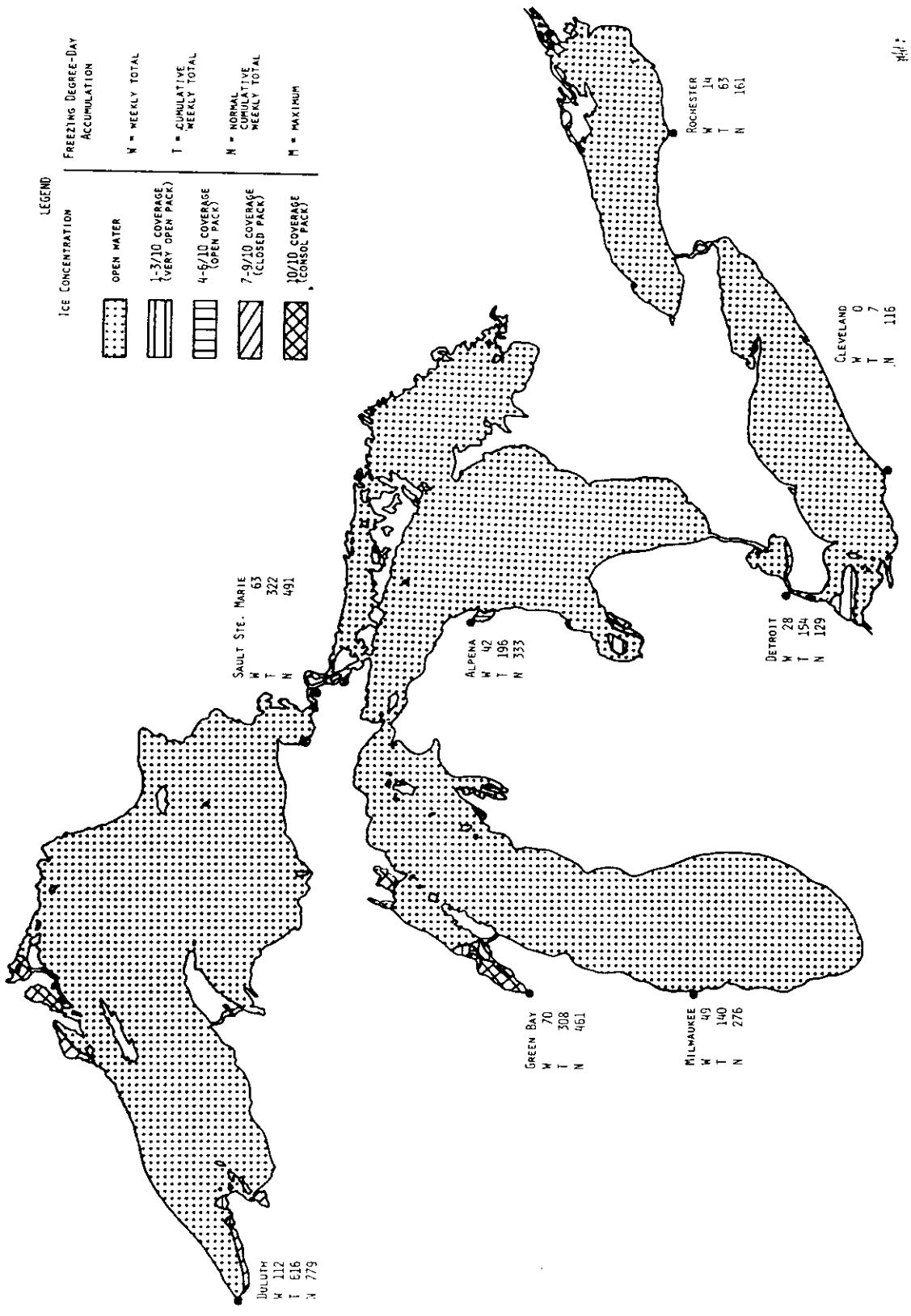
Figure A.9. Composite ice chart - week ending January 5, 1975.
