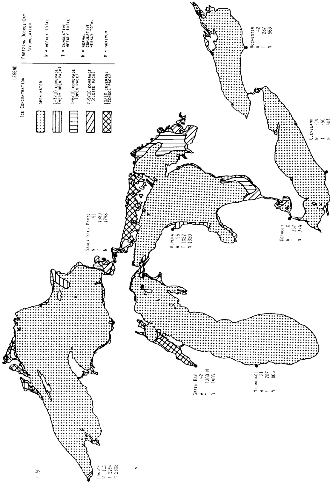
Figure A.22. Composite ice chart - week ending April 6, 1975.
