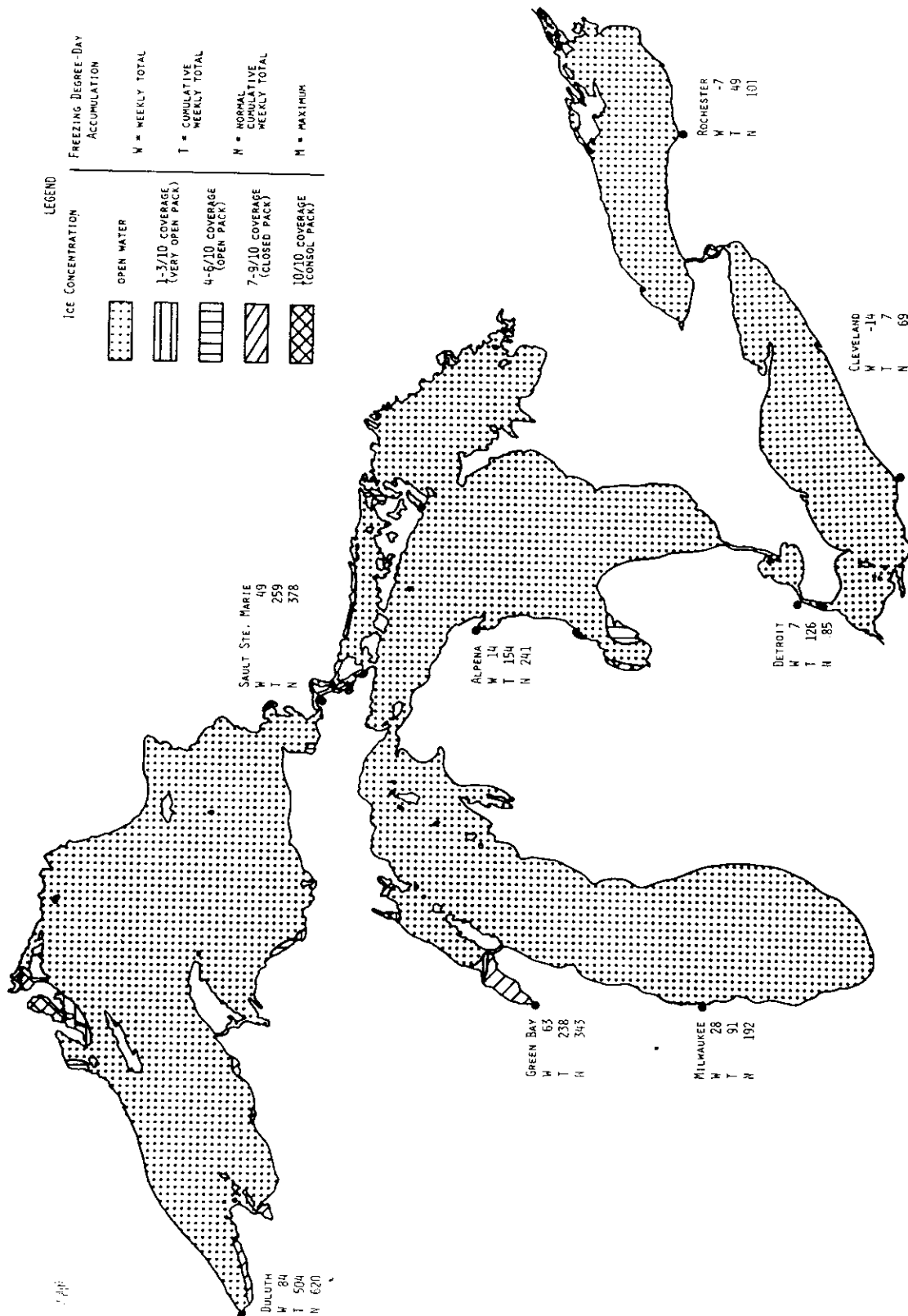
Figure A.8. Composite ice chart - week ending December 29, 1974.
