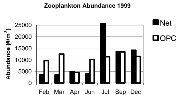
Fig. 4. Zooplankton Abundance – OPC and Nets
