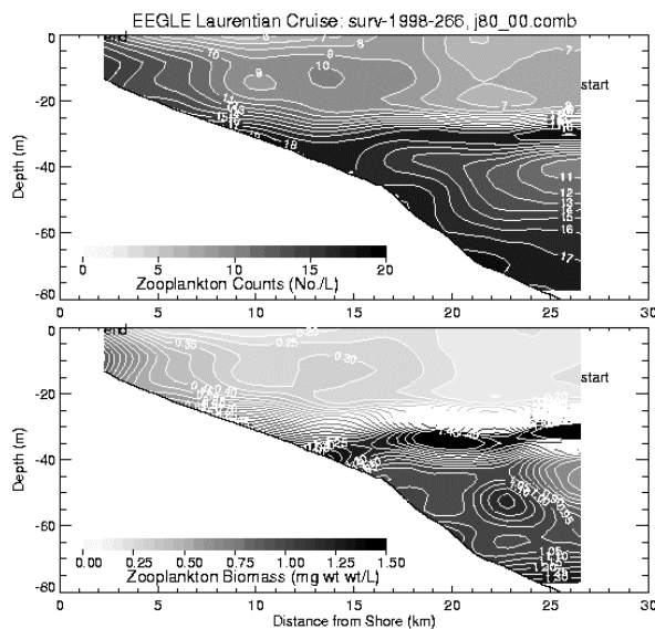
Fig. 8. Zooplankton Abundance and Biomass – Sept. 1998
