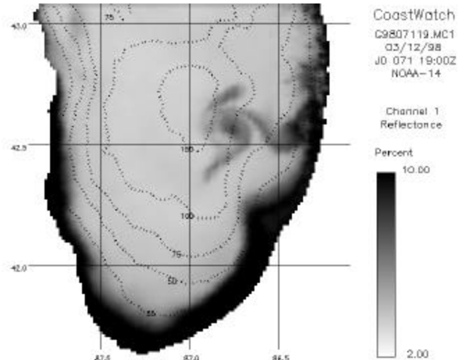
Fig. 6. Sediment Re-suspension Event
