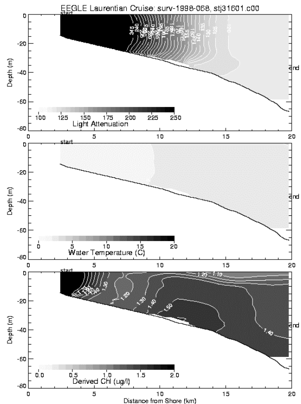
Fig. 7. St. Joseph, MI Transect – March 1998
