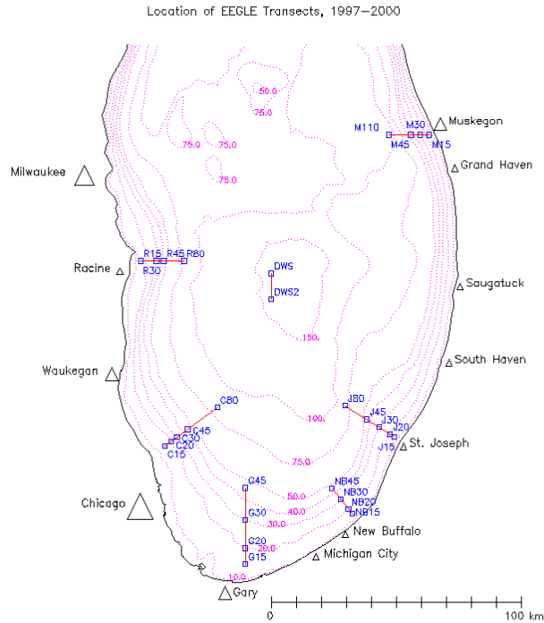
Fig. 2. EEGLE Study Area: Southern Lake Michigan
