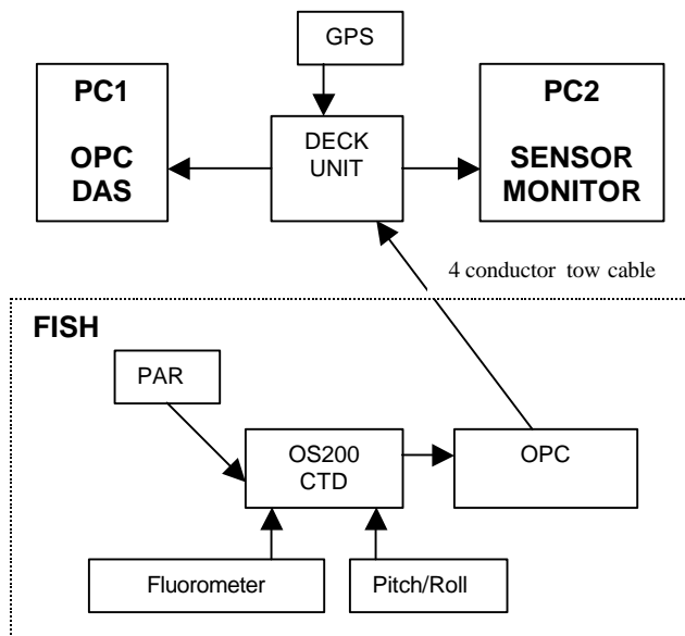
Fig. 1 Simplified block diagram.
