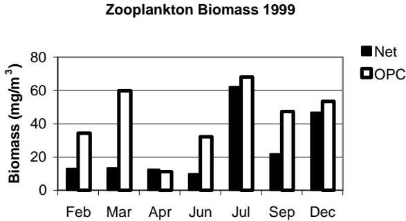
Fig. 5. Biomass – OPC and Nets
