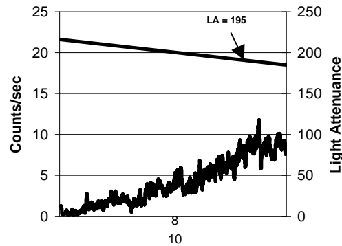
Fig. 3. Zooplankton Counts and Turbidity
